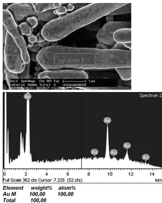
Figure 6: Structural analysis: a) SEM micrograph of Au fibers, b) spectrum of EDS analysis marked as "spectrum 2" in Figure 6a . (Quantification spectrum for the rectangular area in Figure 6a .)
