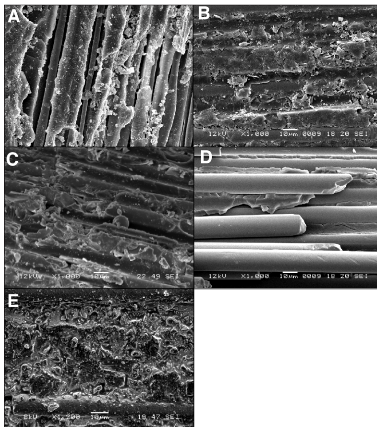
Figure 2: A) Representative SEM micrographs of the fiber post surface after HF etching. Denuded quartz fibers are evident on the post surface, due to deep epoxy resin dissolution (1000x). B) Morphological aspect of the fiber post surface before treatment: no fibers are exposed on the outer surface, which appears embedded in the epoxy resin matrix (1000x bar 10 \mu m). C) SEM images of the fiber post surface after sandblasting (1000x bar 10 \mu m) and D) after etching with 10% hydrogen peroxide for 20 minutes. Exposure of the quartz fibers could be seen as a result of the partial dissolution of the surface epoxy resin. Fibers were not damaged by the etching treatment (1000x bar 10 \mu m). E) SEM image of the experimental zirconium oxide industrial coating: particles are detectable on the post surface, thus covering the fibers and the resinous matrix (1200x bar 10 \mu m).
