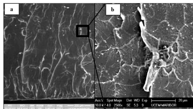
Figure 6: Electron micrographs of the PMMA fracture surface: a) general impression and b) detail
