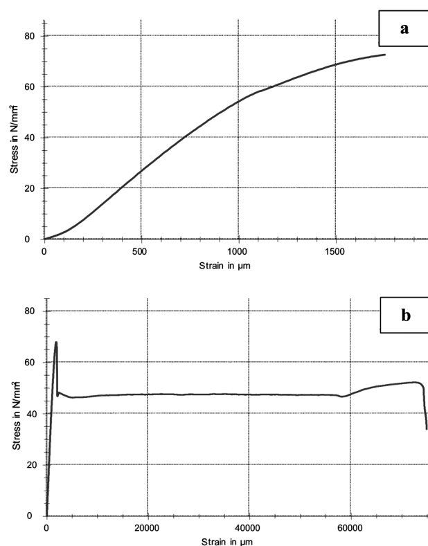
Figure 3: Typical \sigma - \varepsilon curves: a) for PMMA and b) for TPC Slika 3: Značilna krivulja \sigma - \varepsilon : a) PMMA in b) TPC
