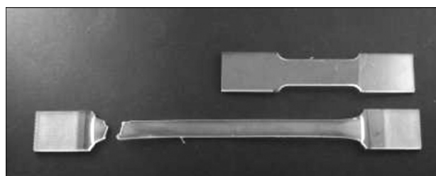
Figure 4: Elongation of the TPC tensile specimens before tensile testing and after the break
