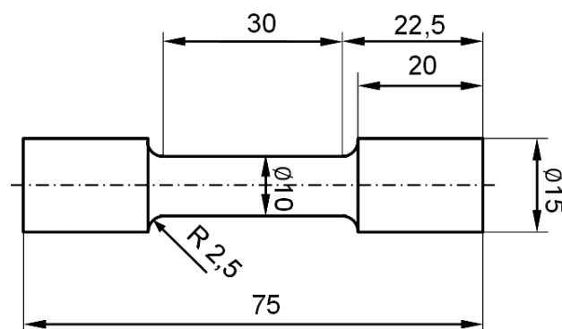
Figure 2: Schematic presentation of a standard tensile-test specimen with dimensions
