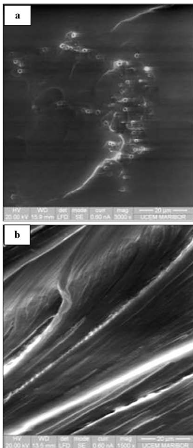
Figure 5: Electron micrographs of: a) PMMA and b) TPC Slika 5: SEM-posnetka: a) PMMA in b) TPC
