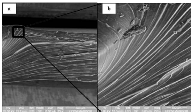
Figure 7: Electron micrographs of the TPC fracture surface: a) general impression and b) detail
