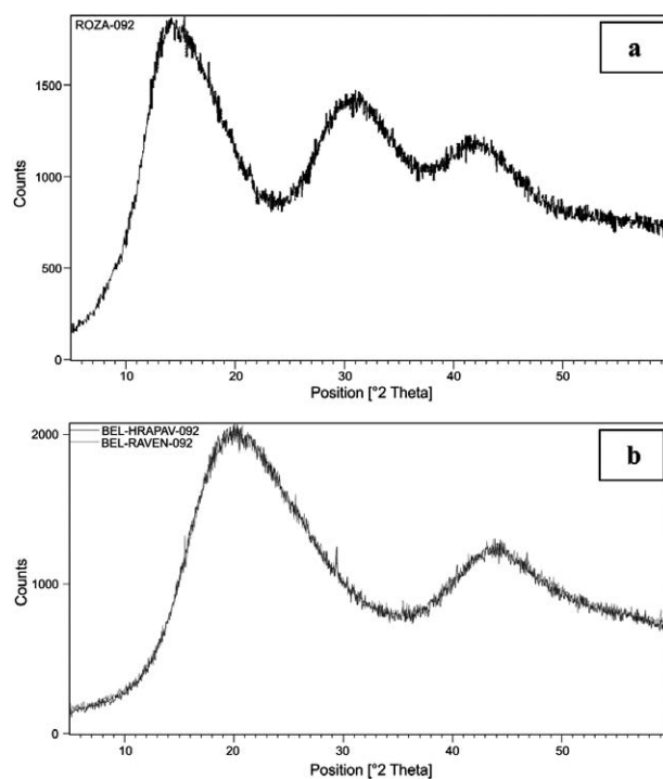
Figure 8: Diffractograms of the samples taken (recorded) from both sides of the plate (rough and smooth) for: a) PMMA and b) TPC
