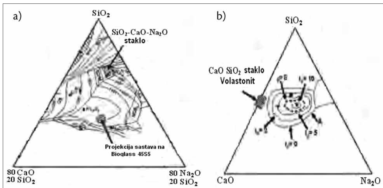
Figure 1. a) \text{SiO}_2 -CaO- \text{Na}_2\text{O} system shows the position of traditional sodium glasses and projection of composition on bioglass 45S5; and b) Section corresponding to the composition of 6% \text{P}_2\text{O}_5 in the system \text{SiO}_2 -CaO- \text{Na}_2\text{O} - \text{P}_2\text{O}_5 and iso-bio-activity lines as a function of composition (wt%) (* bioglass, * 45S5, * cerovital and bioglass) [5].
