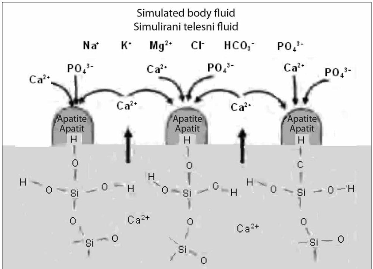
Figure 2. The formation mechanism of carbonated hydroxyapatite layer on A/W glass-ceramics according to Kokubo [16].
